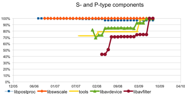
Figure 7. Relative growth in size of S- and P-type components
