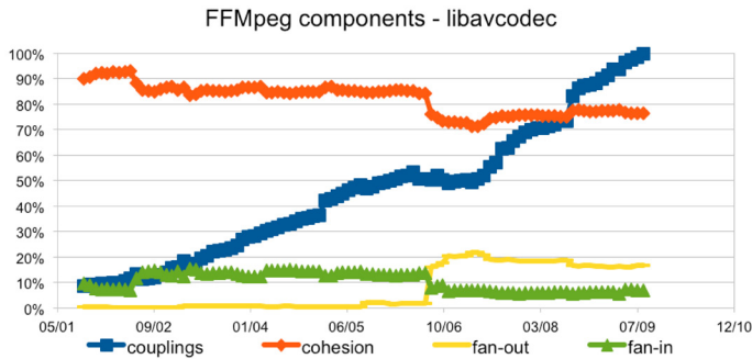
Figure 8. Coupling patterns of E-type components. Libavavcodec.
